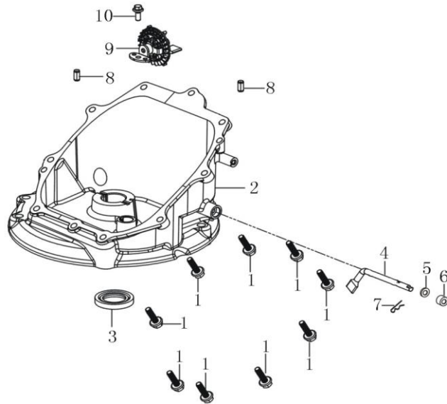
Crankcase cover
